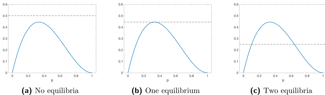
Figure 1: Equilibria of the participation game with n = 4 and threshold w = 2 .
